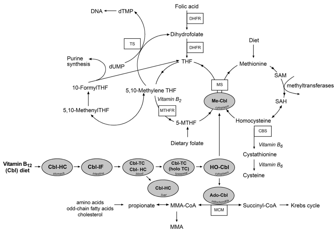
Figure 2. Vitamin B 12 absorption and intracellular processing via two enzymatic pathways. In the absence of vitamin B 12 , 5-MTHF becomes metabolically trapped in this form producing a pseudo folate-deficient state (methyl-trap) and cannot be utilized for regeneration of THF. Cbl: cobalamin; CBS: cystathionine beta-synthase; dTMP: deoxythymidine monophosphate; dUMP: deoxyuridine monophosphate; DHFR: dihydrofolate reductase; HC: haptocorrin; holoTC: holotranscobalamin; HO-Cbl: hydroxocobalamin; IF: intrinsic factor; MS: methionine synthase; Me-Cbl: methylcobalamin; MTHFR: methylene tetrahydrofolate reductase; MMA: methylmalonic acid; MCM: methylmalonyl-CoA mutase; 5-MTHF: 5-methyltetrahydrofolate; SAH: S-Adenosyl homocysteine; SAM: S-Adenosyl methionine; THF: tetrahydrofolate; TS: thymidylate synthase; TC: transcobalamin.
