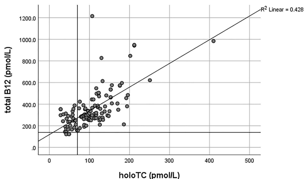
Figure 5. The correlation between holoTC and serum B 12 in the holoTC range \geq 25 pmol/L. The horizontal line on the y-axis represents the serum B 12 deficiency cutoff of 138 pmol/L and the vertical line represents the holoTC cutoff of 70 pmol/L for B 12 replete patients as used in authors' laboratory (AS-M and DJH). Samples with holoTC results between 25–70 pmol/L are referred for additional testing.
