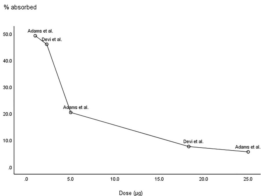
Figure 3. Relationship between the intake and percentage of absorbed B 12 from a dose of [ 58 Co]-cyanocobalamin (Adams et al. [34]) and [ 13 C]-cyanocobalamin (Devi et al. [35]) in n = 10–12 healthy volunteers.
