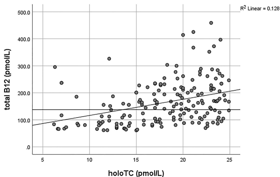
Figure 4. The correlation between holoTC and serum B 12 in the low holoTC range, <25 pmol/L. The horizontal line on the y-axis represents the serum B 12 deficiency cutoff of 138 pmol/L used in the authors’ laboratory (AS-M and DJH).
