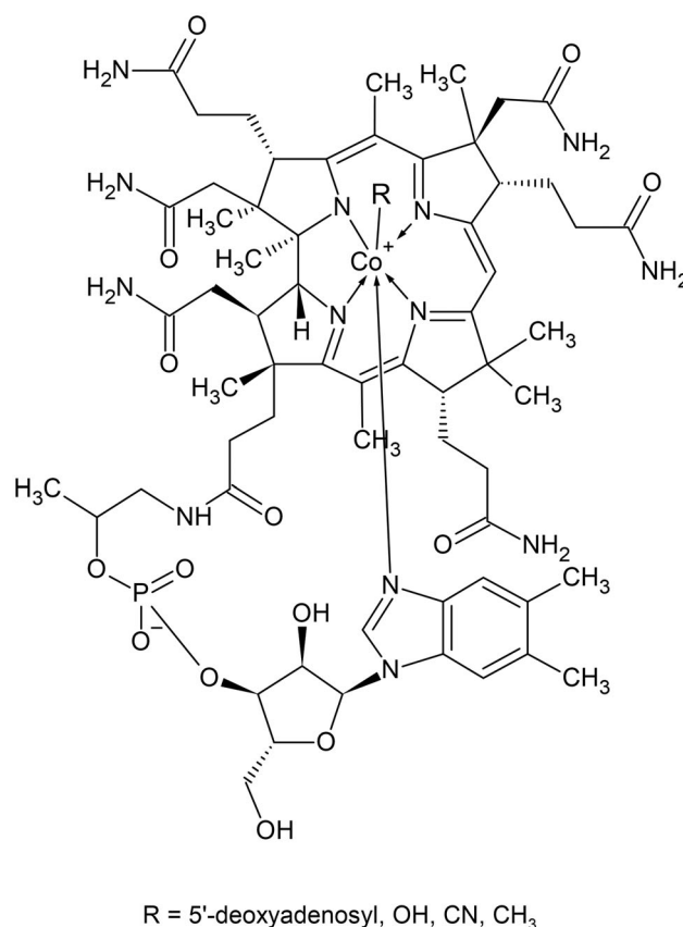
Figure 1. The chemical structure of vitamin B 12 .
